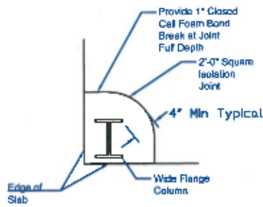
Typical Column at Corner of Building
