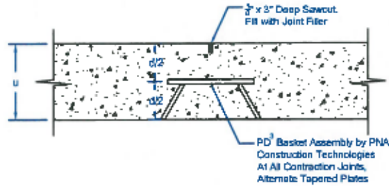
Typical Construction Joint
