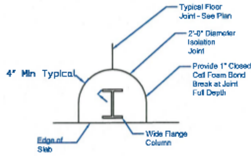
Typical Column at Edge of Building
