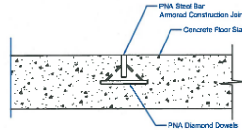
Armored Construction Joint
