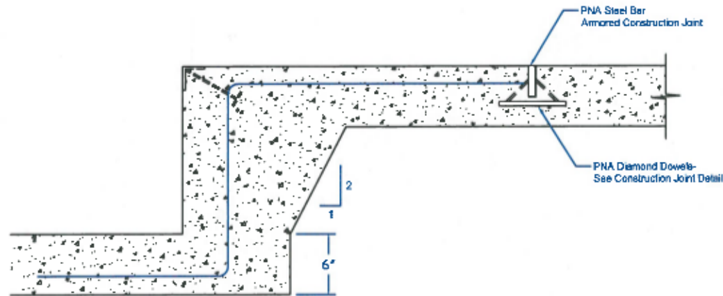
Typical Dock Leveler Pit
